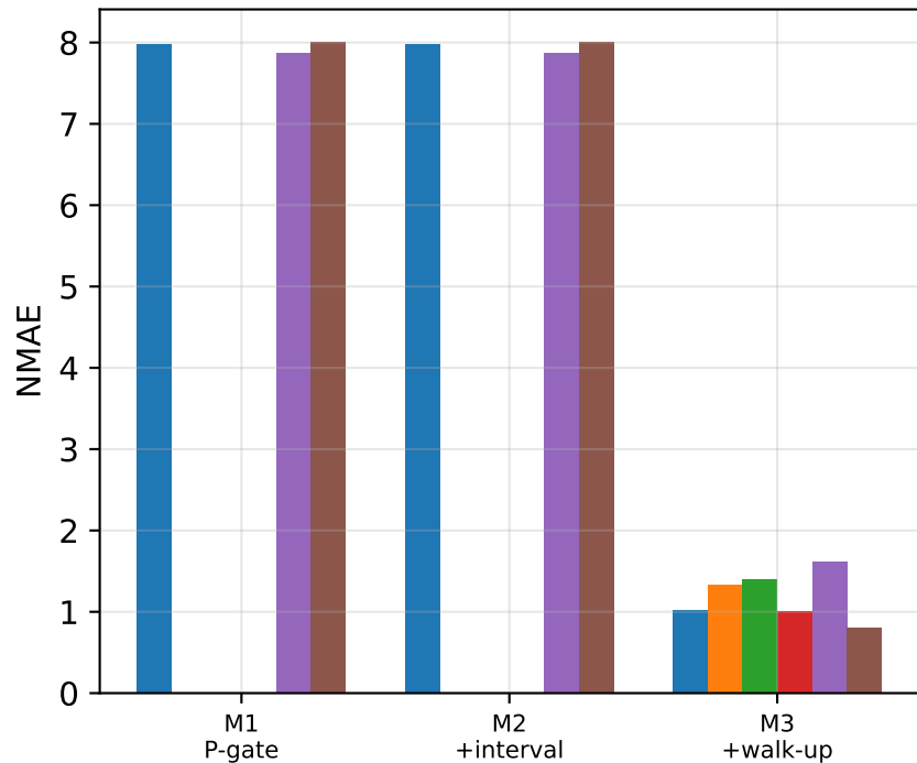
(b) Walk-up collapses leaf NMAE
