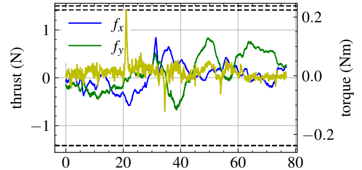
Commanded Force and Torque
