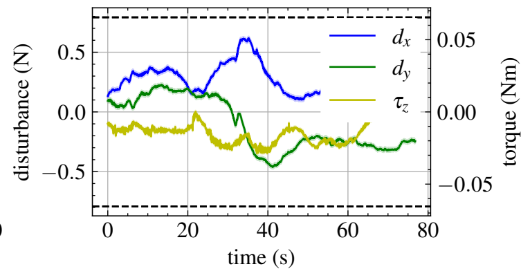
Estimated Disturbance
