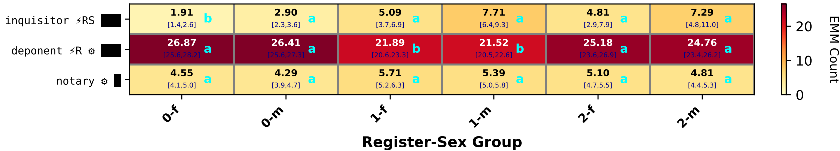
Panel 1: Estimated Marginal Means (HC3 Robust) with 95% CIs & CLD (FDR-corrected)
