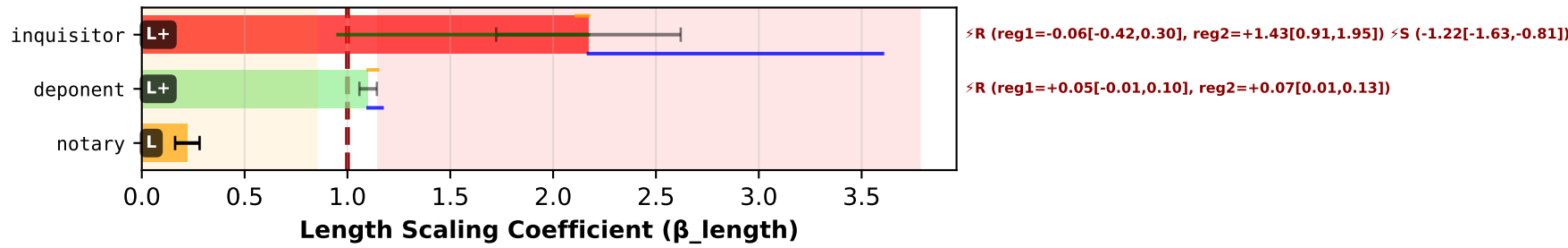
Panel 2: Length-Content Relationship (bar=baseline 0-f, black=95% CI) Interaction lines: Orange=reg1 | Blue=reg2 | Green=sex | ↗R/S=coeffs+Cls (right)
