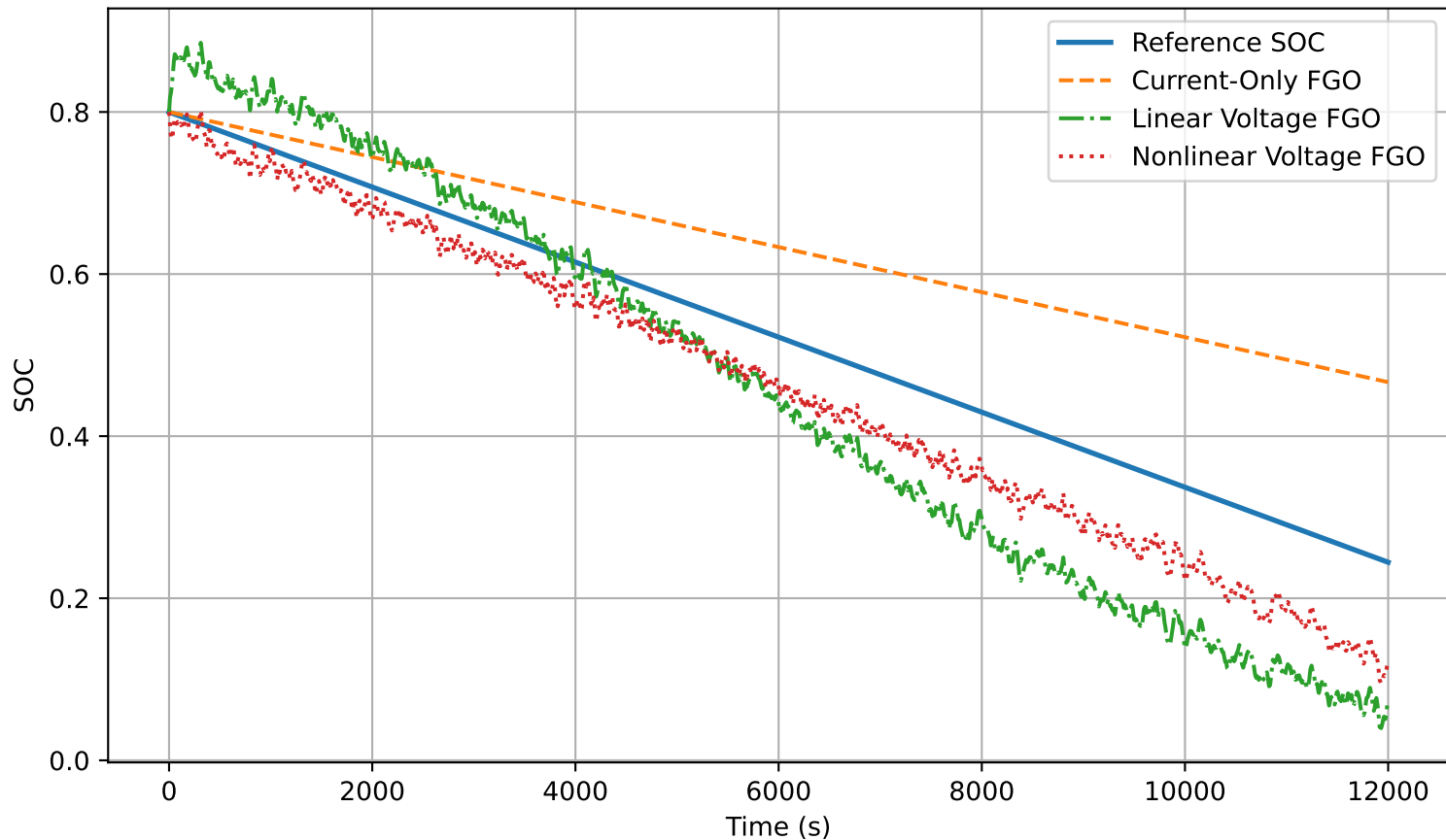
SOC Estimation Comparison under Constant-Current Conditions
