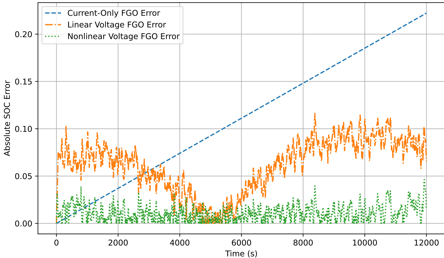
SOC Estimation Error under Constant-Current Conditions
