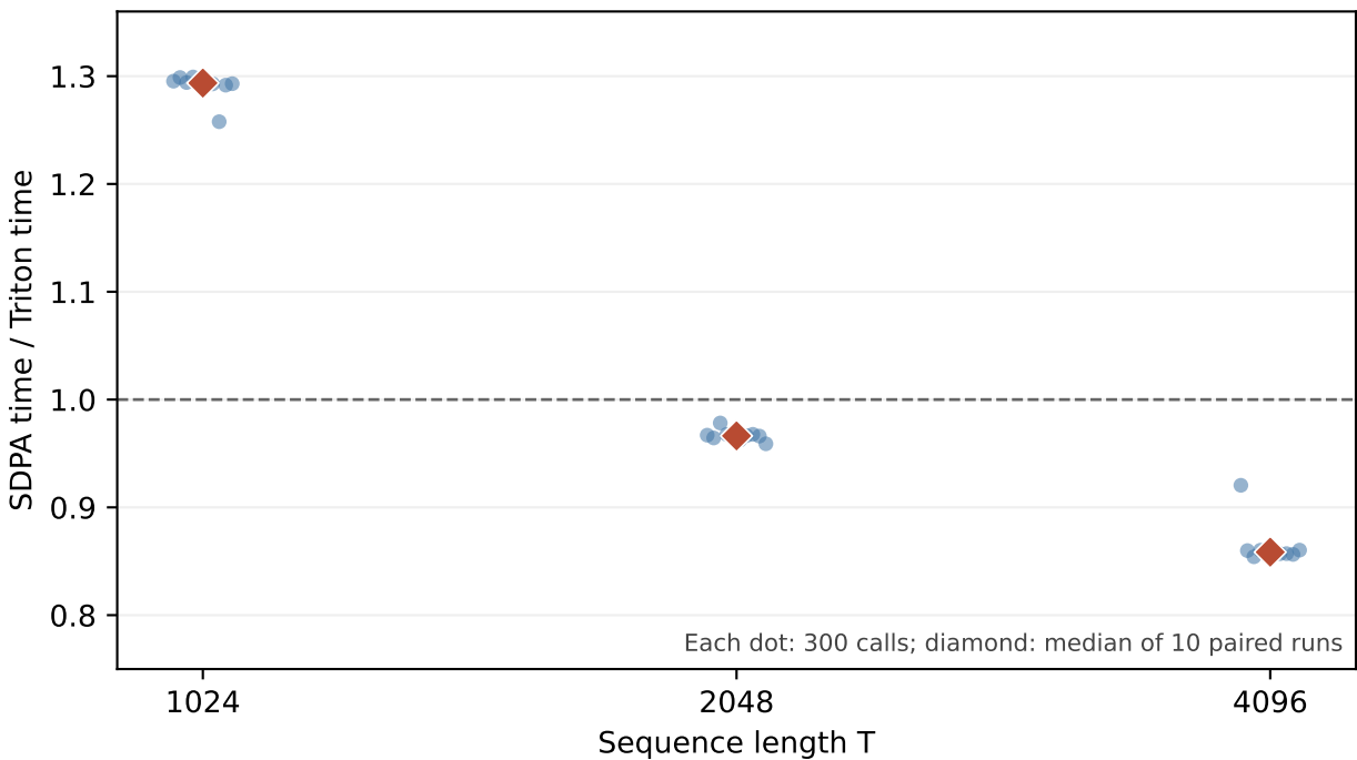
RTX 4090 causal attention forward (CUDA events)
