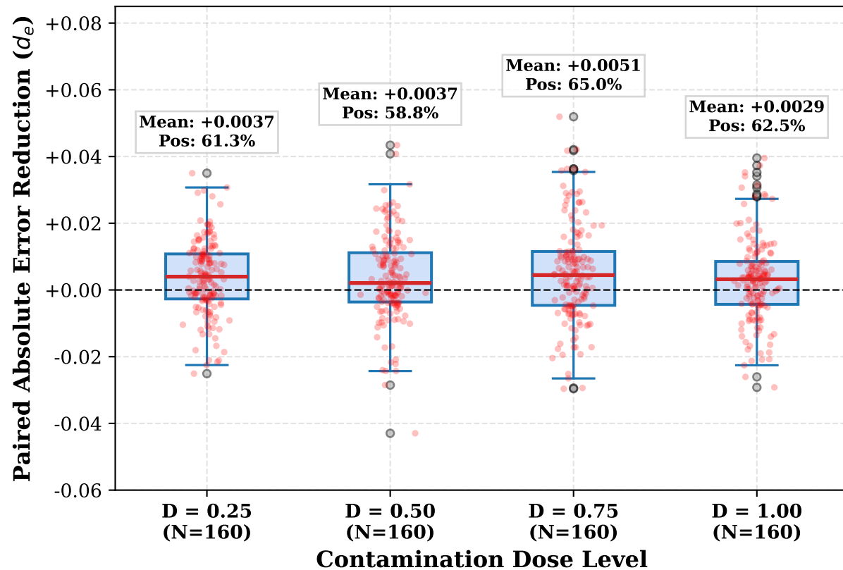
(A) Event Error Reductions by Contamination Dose
