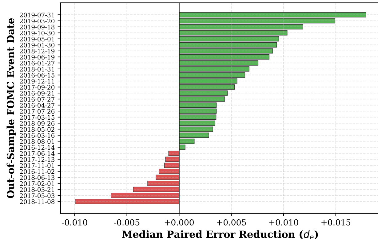
(B) Event Heterogeneity Across 32 OOS Meetings
