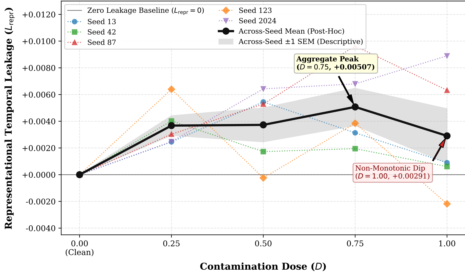
Figure 1: Representational Temporal Leakage Dose-Response Curve Substantial Positive Shift with Seed Heterogeneity & Non-Monotonic Peak
