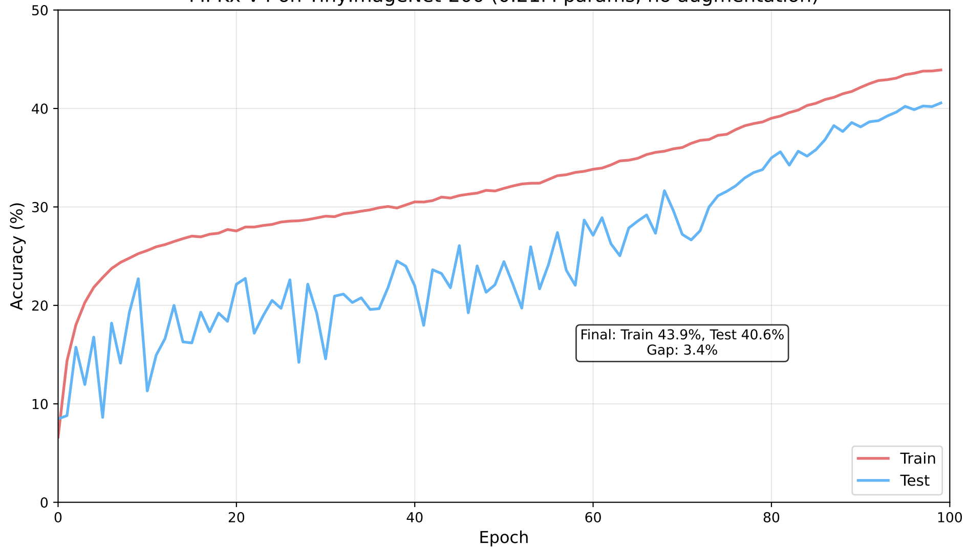
MPKx V4 on TinyImageNet-200 (0.21M params, no augmentation)
