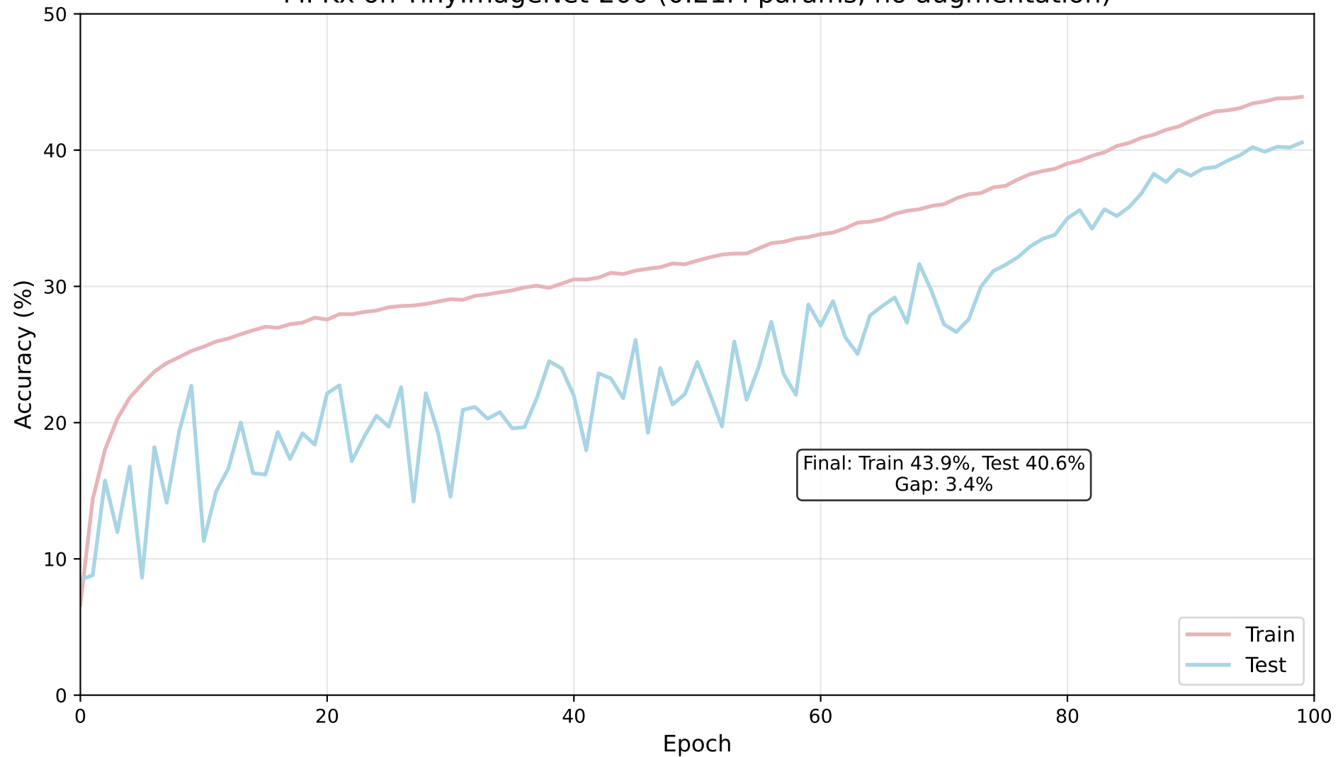
MPKx on TinyImageNet-200 (0.21M params, no augmentation)
