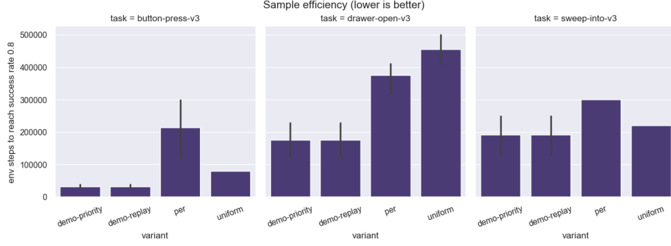
Figure 13: Env-steps to first 0.8 success-rate crossing on each MetaWorld task, by replay-buffer variant. Bars show the mean over seeds that reached 0.8 within the 500k step budget; the “ n/5 ” annotation indicates how many seeds reached the threshold. Both demo variants reach 0.8 in all five seeds on every task, including sweep-into-v3 where the policies later collapse—demos solve the first-touch exploration problem but not the stability problem on harder tasks.
