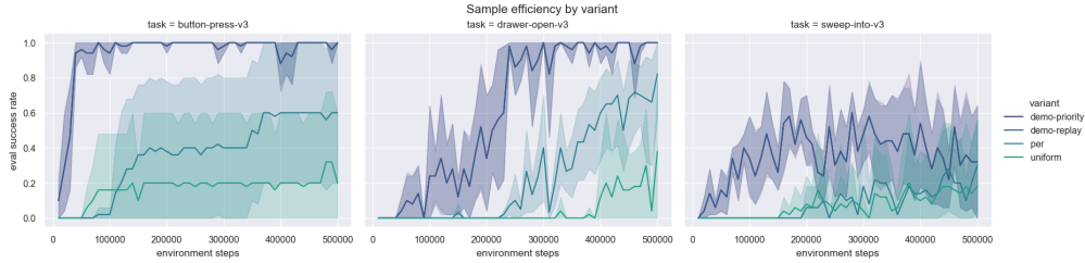
Figure 14: Evaluation success-rate curves over training, by replay variant and task. Solid line is the seed mean, shaded band is the 95% bootstrap CI across the 5 seeds. The demo-replay and demo-priority curves are visually indistinguishable on every panel—they are in fact bit-identical (§H.3). PER consistently outruns uniform across all three tasks.
