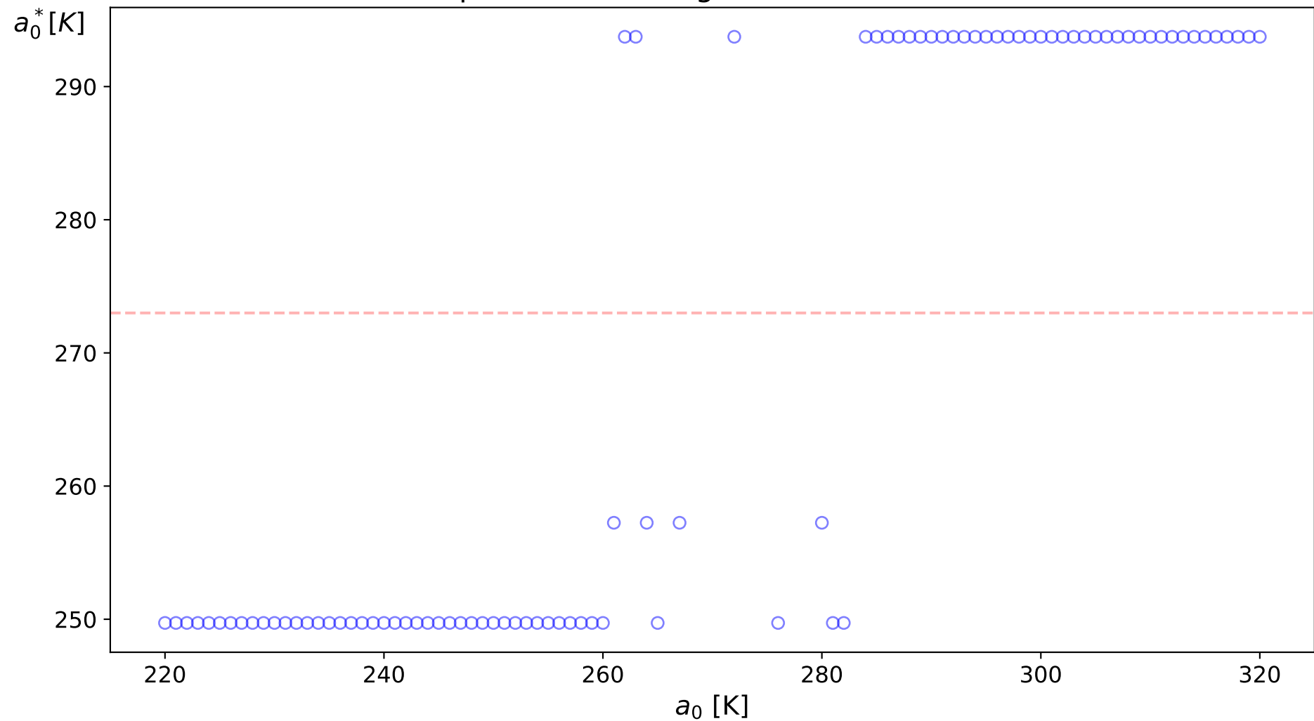
Climate Equilibria: Converged Solution vs Initial Guess
