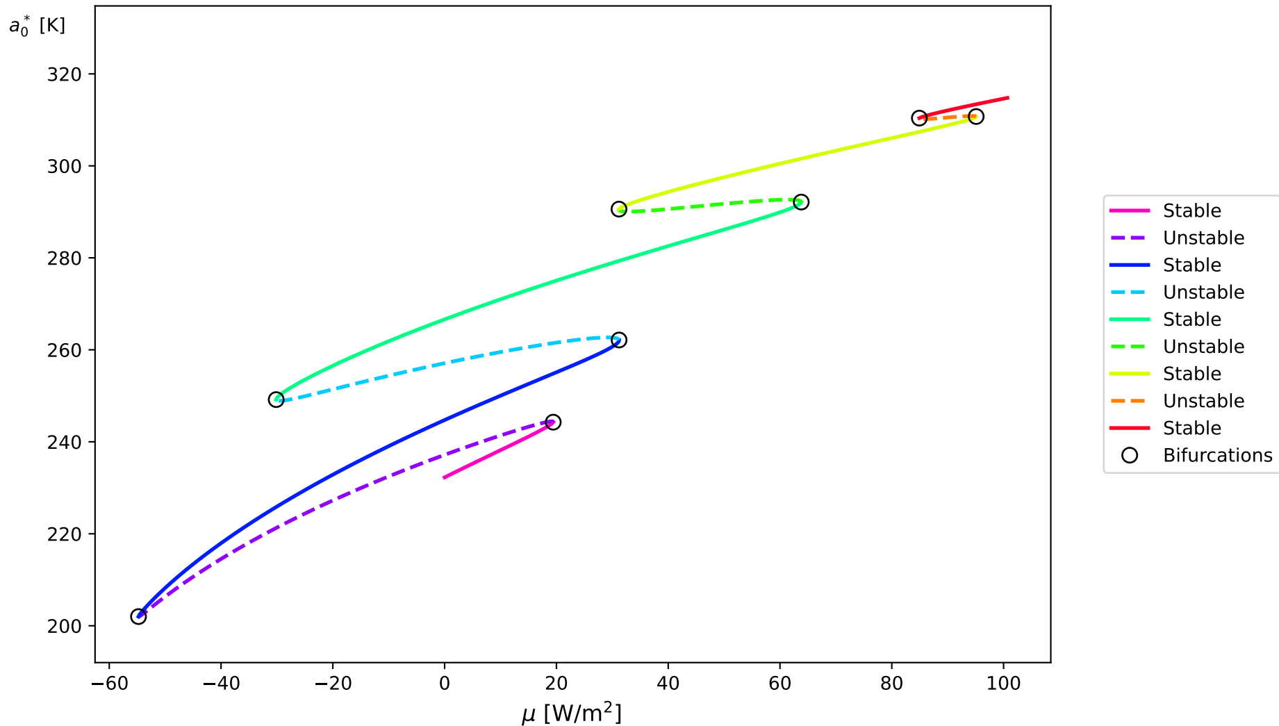
Bifurcation Diagram ( D = 0.003 )
