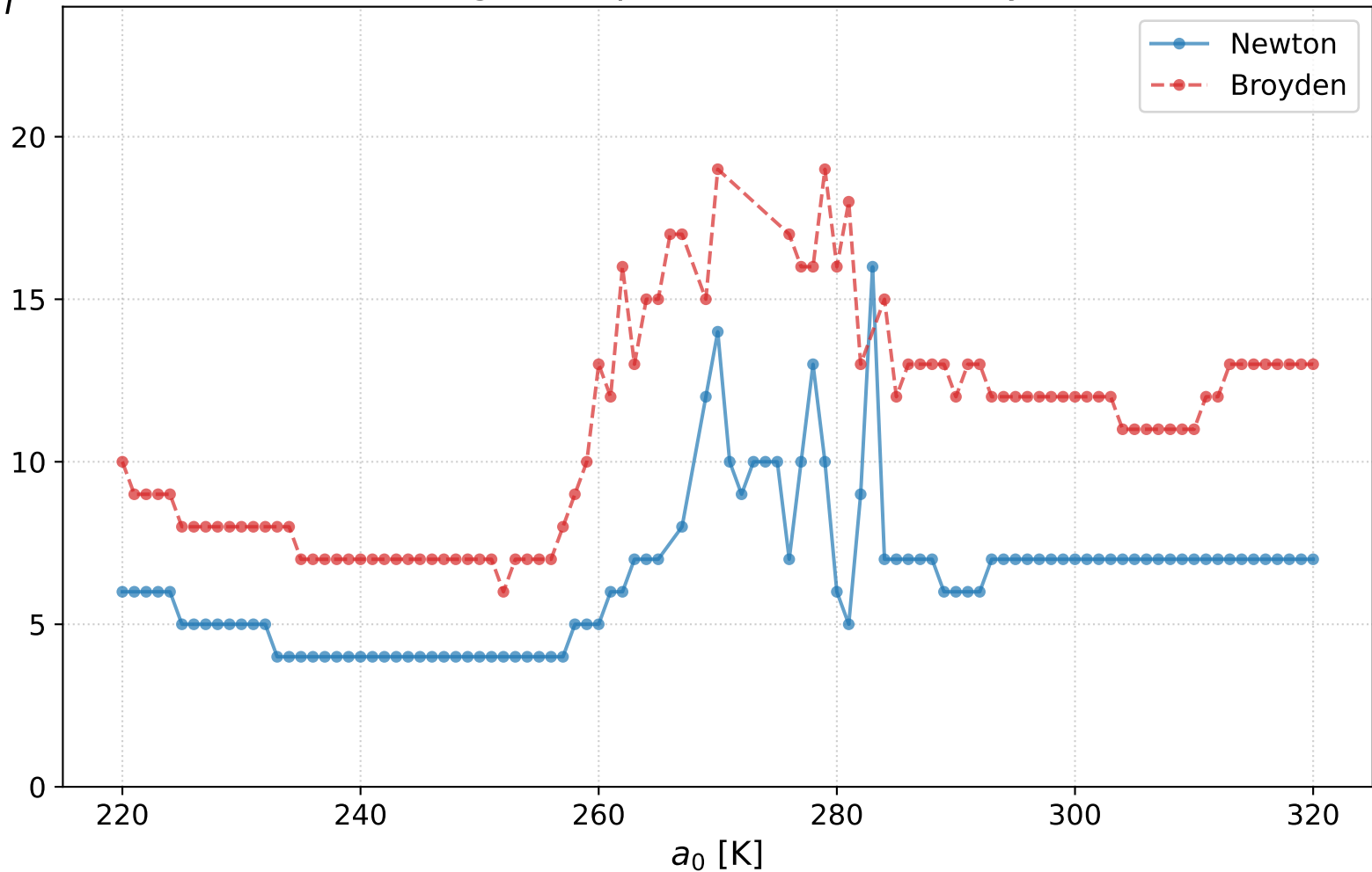
Convergence speed: Newton vs Broyden
