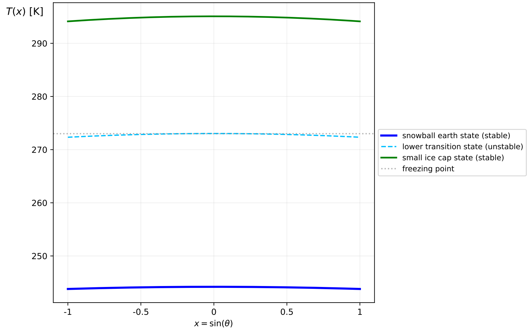
Global Temperature Profiles around \mu = 20.0 \text{ W/m}^2
