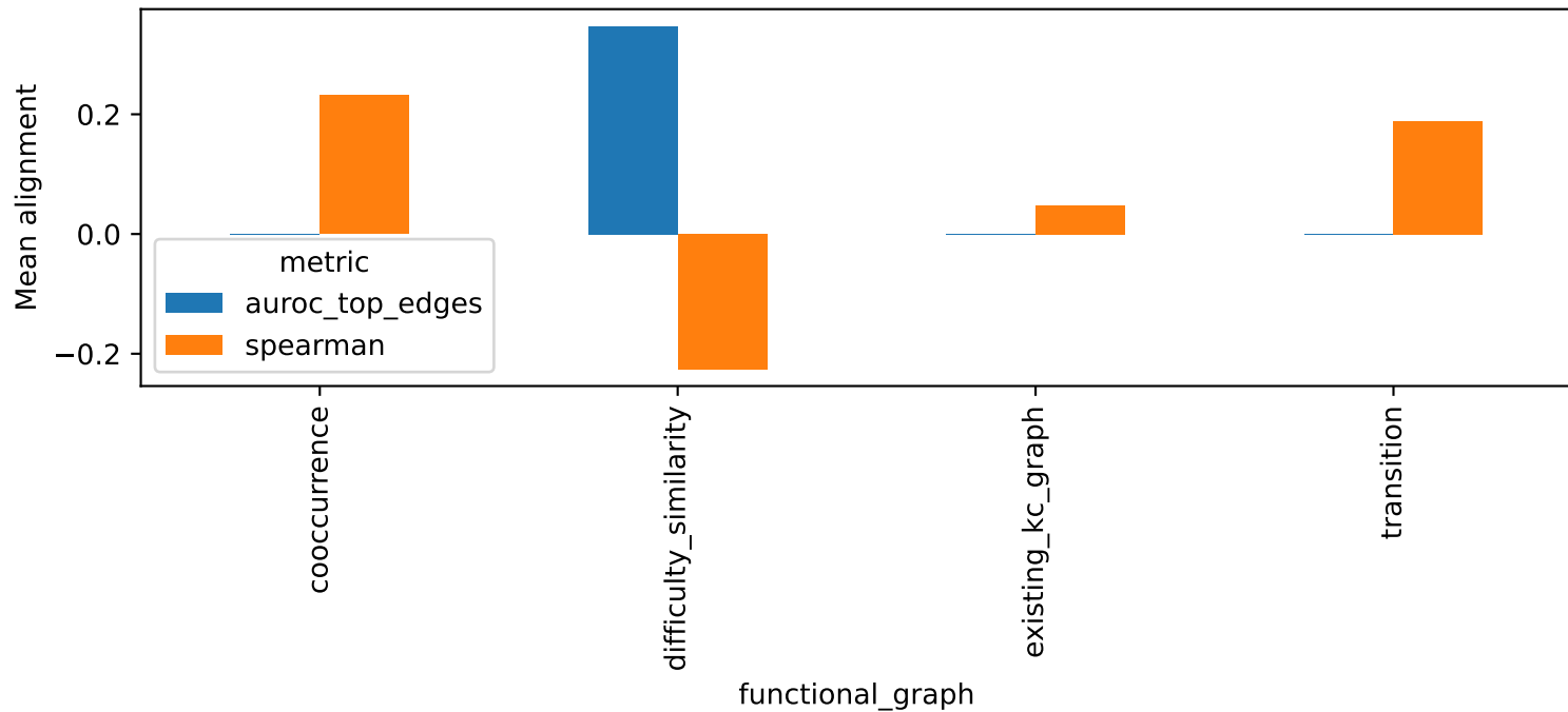
Semantic prototype vs functional graph alignment
