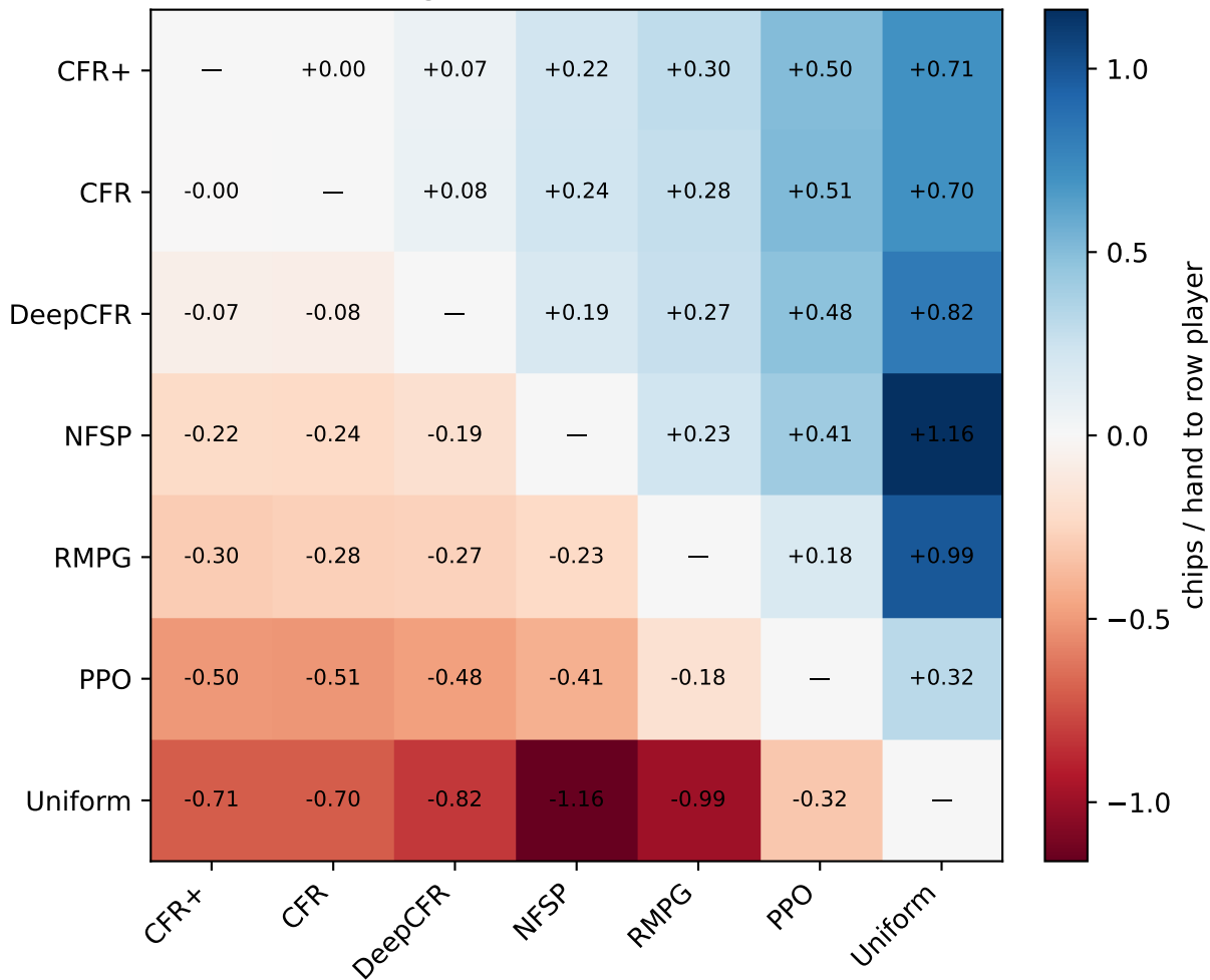
Head-to-head: chips/hand, row vs column (seat-averaged, exact; + means row wins)
