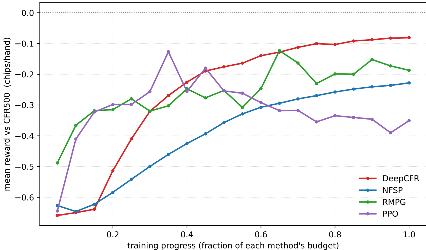
Mean reward vs CFR500
