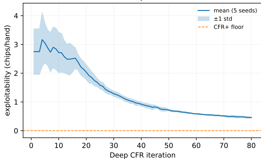
DeepCFR
