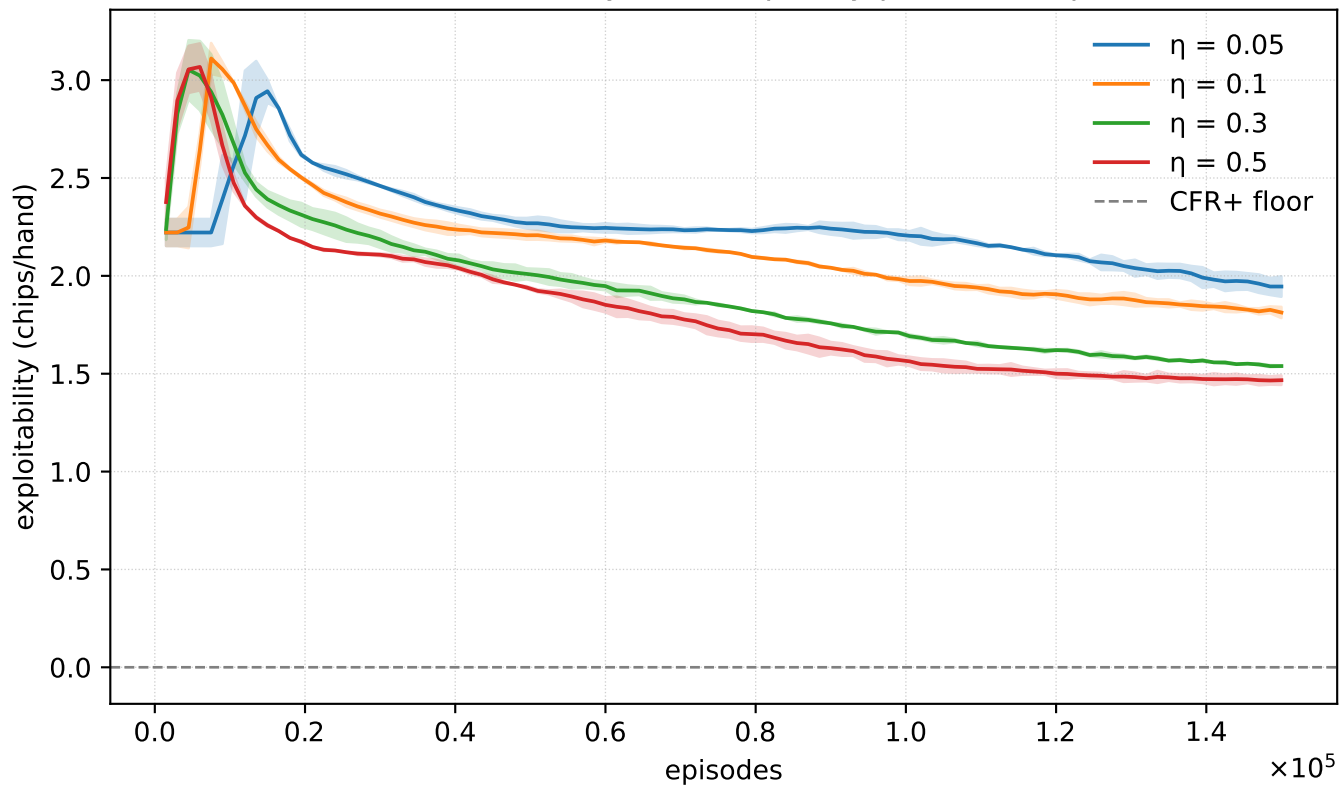
NFSP sensitivity to anticipatory parameter \eta
