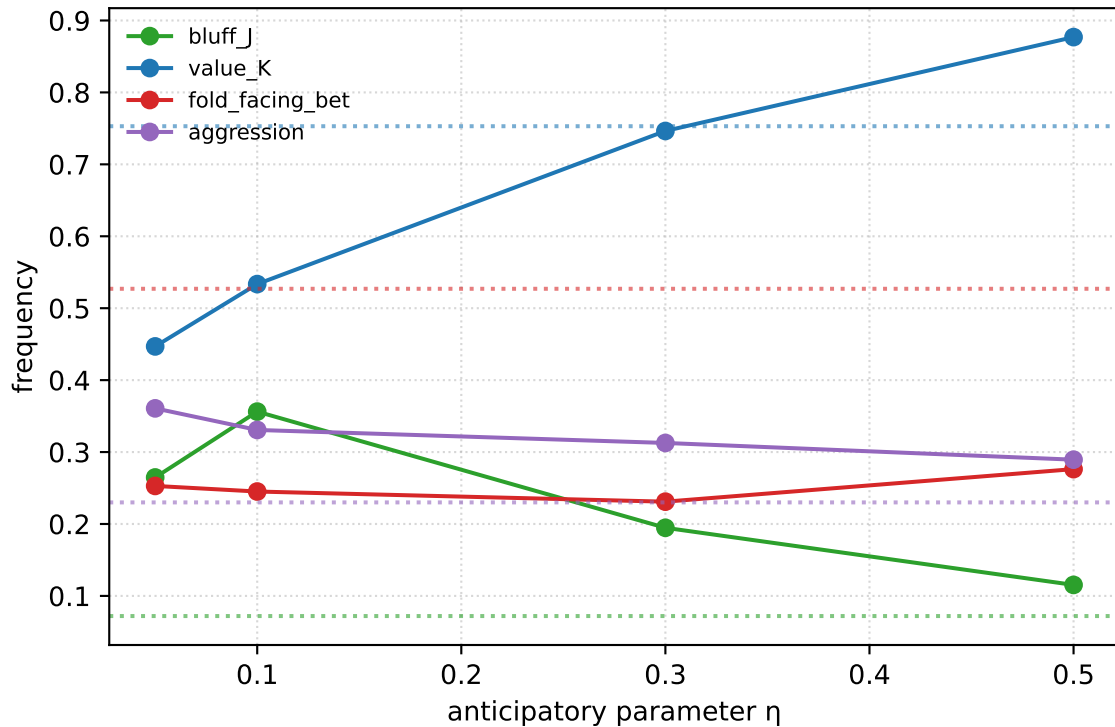
NFSP behaviour vs \eta (dotted = CFR+)
