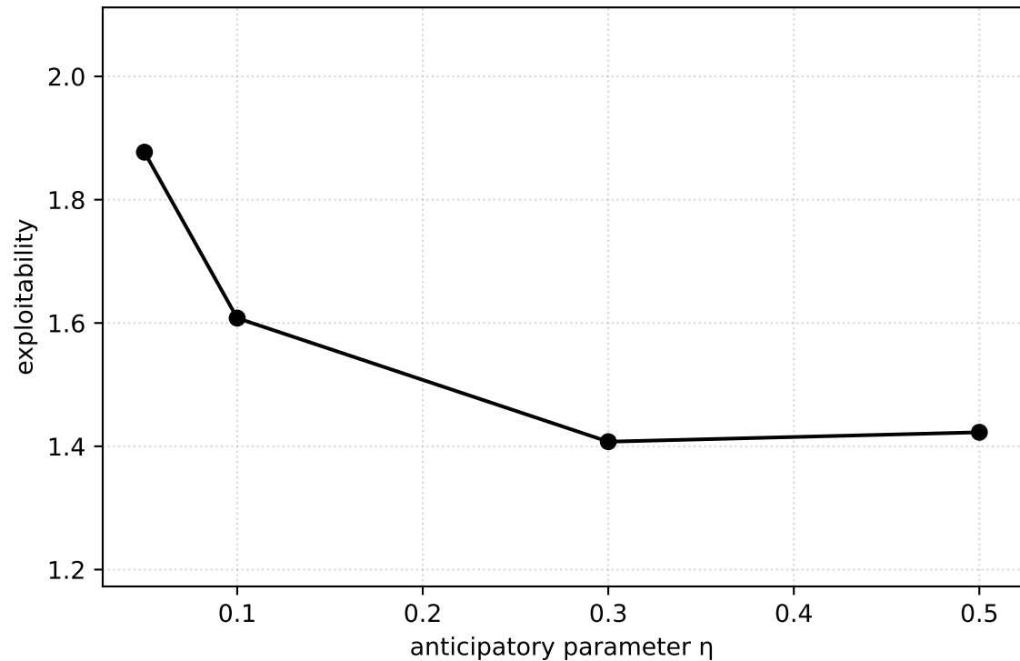
NFSP exploitability vs \eta
