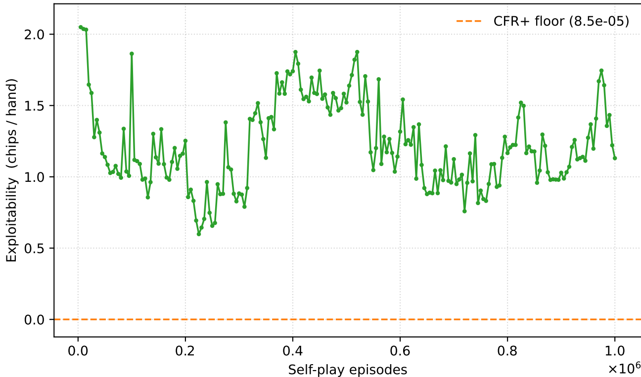
RMPG current-policy exploitability
