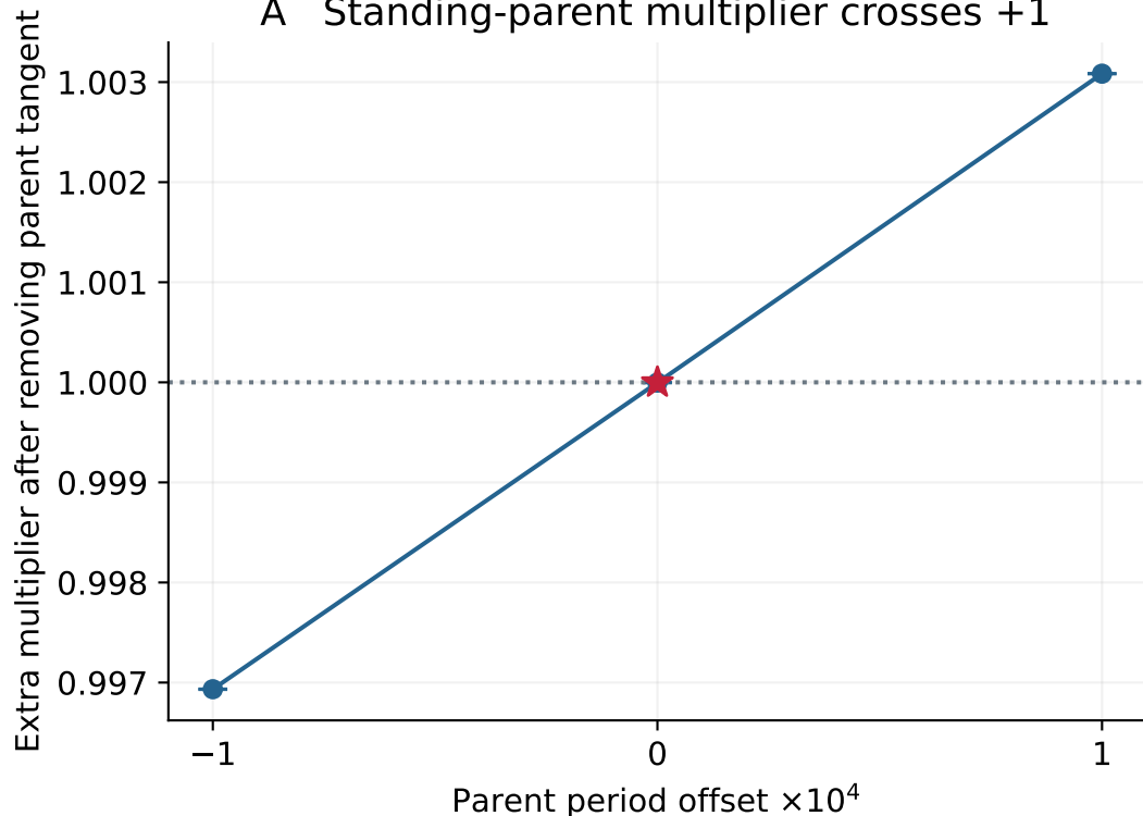
A Standing-parent multiplier crosses +1
