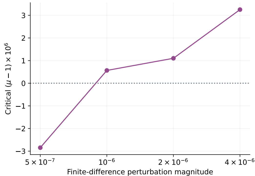
B Numerical resolution at the critical orbit
