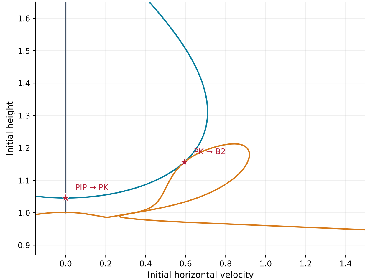
Zoom on the verified PIP \rightarrow PK \rightarrow B2 route
