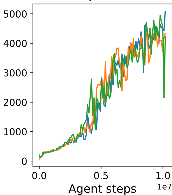
Q*bert
