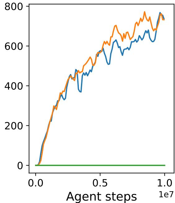
Enduro
