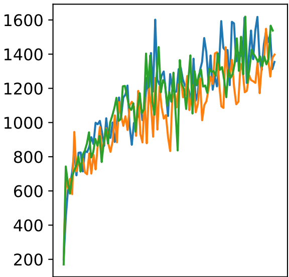
MsPacman
