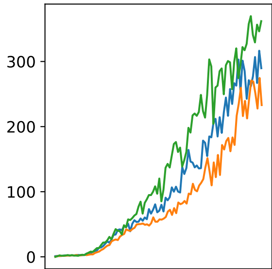
Breakout
