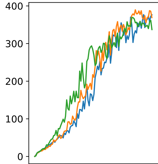
Breakout
