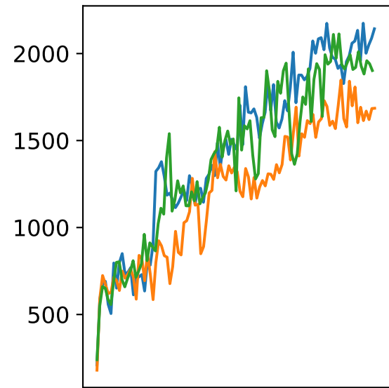
MsPacman
