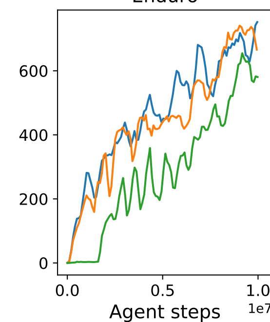
Enduro
