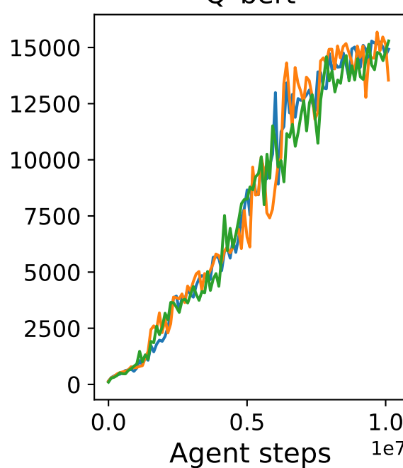
Q*bert
