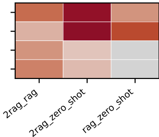
Mistral Small
