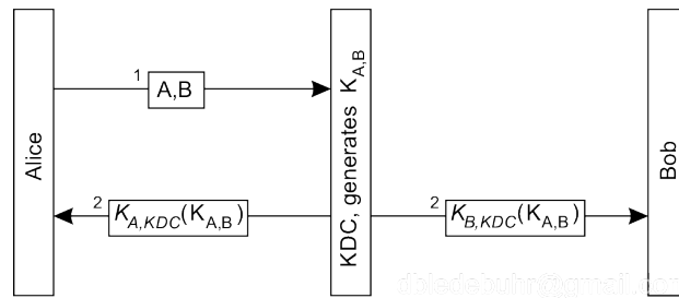
Figure 9.9: The principle of using a Key Distribution Center (KDC).
