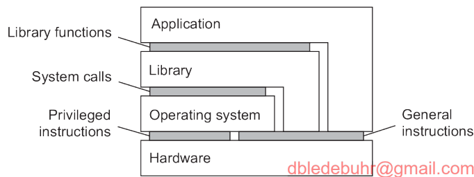
Figure 3.7: Various interfaces offered by computer systems.
