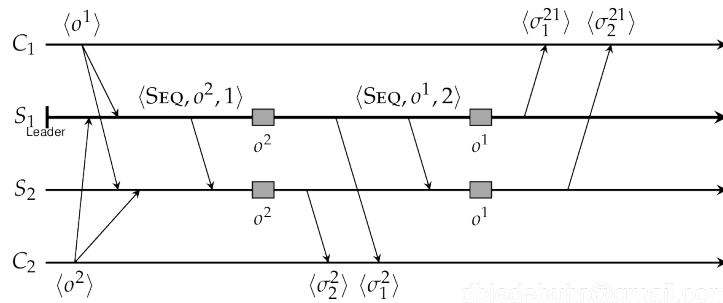
Figure 8.7: Two clients communicating with a 2-server process group.
