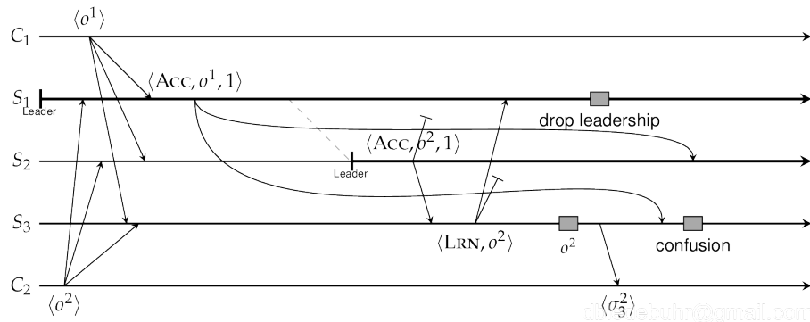
Figure 8.11: Why incorporating the ID of the current leader is needed.
