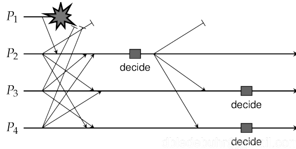
Figure 8.5: Reaching consensus through flooding in the presence of crash failures. Adopted from ?.
