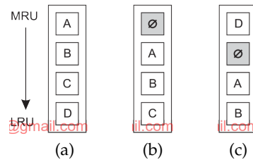
Figure 3.2: The organization of the cache when dealing with interrupts: (a) before the context switch, (b) after the context switch, and (c) after accessing block D. (Adapted from ?.)
