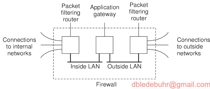
Figure 9.22: A common implementation of a firewall.
