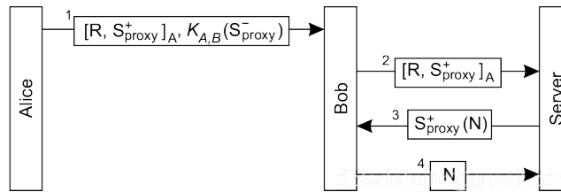
Figure 9.32: Using a proxy to delegate and prove ownership of access rights.
