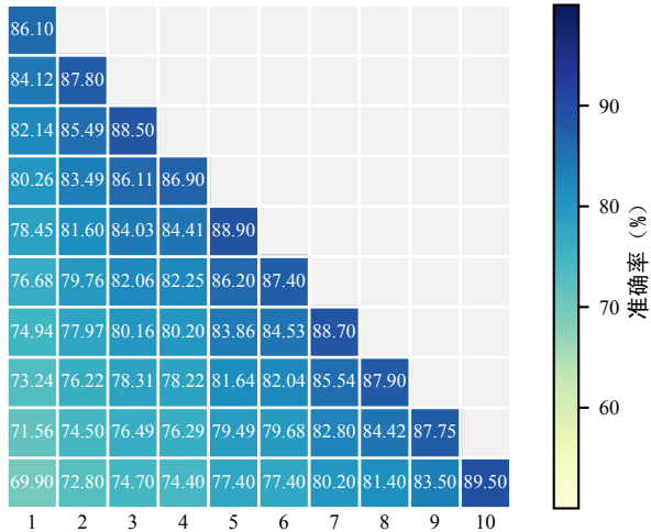
FedSubMerge-AD
