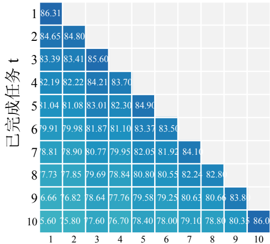
FedSubMerge
