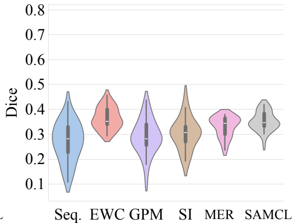
(b) Abdomen CT-CT
