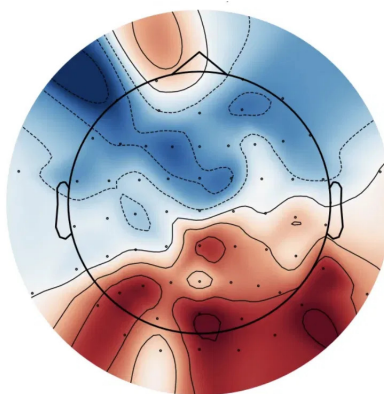
Figure 10: Haufe-transformed forward pattern for the rpCond versus swCond decoder, 150 to 250 ms ( N = 58 ). Warm values are swCond-like and cool values rpCond-like; solid and dashed contours mark positive and negative values. Units are arbitrary, since forward patterns are defined up to scale.
