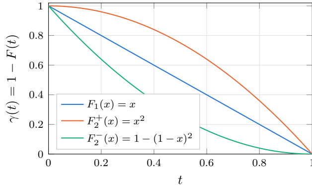
Figure 16: The profiles behind Figure 15: the survival function \gamma(t) = 1 - F(t) of each statistic, which by (93) is the mean entropy of a fresh answer at macroscopic time t . Convex, straight and concave F give concave, straight and convex profiles; the smaller of two draws spends its predictive power earliest, the larger of two hoards it.
