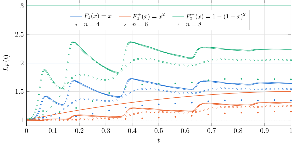
Figure 15: The two families of (95) and (97) at r = 2 , meeting at r = 1 ; their profiles are in Figure 16. The larger of two draws ( F_2^+(x) = x^2 , orange) delays its deductions and climbs from the baseline to L_2^+(1) = \frac{3}{2} ; the smaller of two draws ( F_2^-(x) = 1 - (1 - x)^2 , green) holds the constant L_2^- \equiv 3 ; between them lies the single uniform draw ( F_1(x) = x , blue), the one statistic the families share, at L \equiv 2 . Dots are finite- n leverage: filled n = 4 (all 2^{16} question sets enumerated, exact), circles n = 6 and triangles n = 8 (Monte Carlo over question orders, subset entropies exact via the nested rank profile, latent-label information included). Convergence is slow from below: the label costs O(\log n) of the Q available bits, and the mean rate approaches its limit only as 1/\sqrt{n} . The left edge is a boundary layer: L_F(0^+) = 1 + f(0^+) presumes 1 \ll \ell \ll Q , while at \ell = 1 the only exhaustible class is the constants and \langle L_1 \rangle = 1 + (Q - 1)w_0^2/(2 \ln 2) + O(w_0^3) , the early deductions being spent on identifying the latent label. The finite curves also scallop, most visibly at n = 8 : each surge is one class being learned out near its rate K_d/Q , a discreteness the limit smooths away as the rate grid refines.
