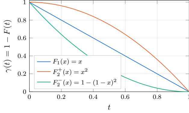
Figure 16: The increment profiles behind Figure 15: the survival function \gamma(t) = 1 - F(t) of each statistic. By (111) it is the mean entropy (expected surprisal) of one fresh answer at macroscopic time t . Convex, straight and concave F give concave, straight and convex profiles respectively; the smaller of two draws spends its predictive power earliest, the larger of two hoards it.
