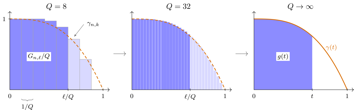
Figure 14: From the finite increments to the profile. Each bar has width 1/Q and height \gamma_{n,k} , so the shaded bars sum, the telescoping identity (88), to exactly G_{n,\ell}/Q , here at t = \ell/Q = 5/8 . Refining Q shrinks the bars onto the staircase’s limit, and dominated convergence turns the shaded sum into the area g(t) = \int_0^t \gamma : received information per question becomes the dark area under the profile.
