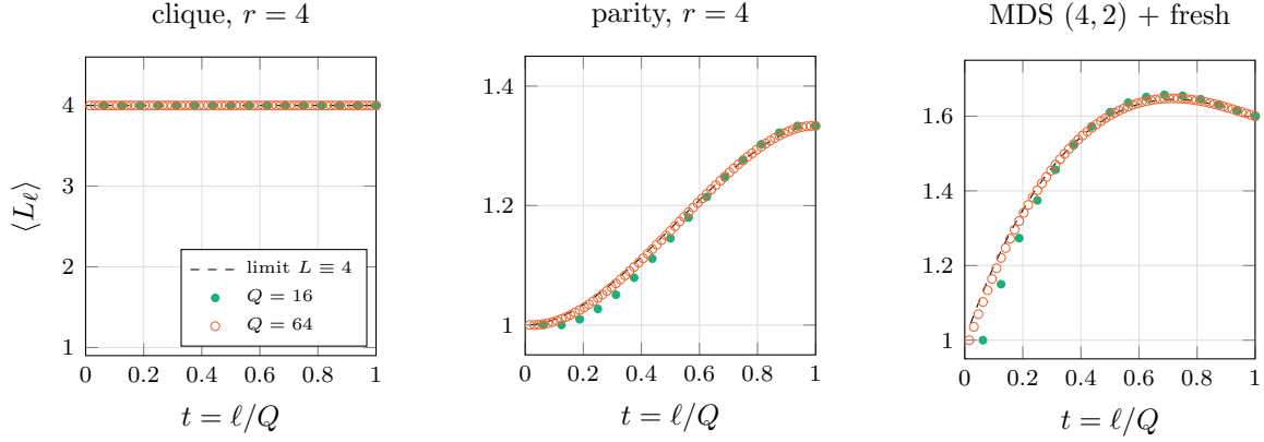
Figure 22: Exact finite- n leverage (dots, Q = 16 and 64 ) against the macroscopic limits (dashed), from (137) and (86) with no simulation. Left: cliques of four with a fair shared bit; the dots sit exactly on the constant L \equiv 4 at every finite n . Middle: parity blocks of four; deductions concentrate late and the finite curves approach the rise to r/(r-1) = \frac{4}{3} from below. Right: a 3:1 mixture of [4, 2] MDS code blocks ( m = 2 ) with fresh questions; the code releases its deductions around the threshold and the fresh sites keep receiving afterwards, an interior maximum of 1.645 at t \simeq 0.72 against the completion value 1.6.
