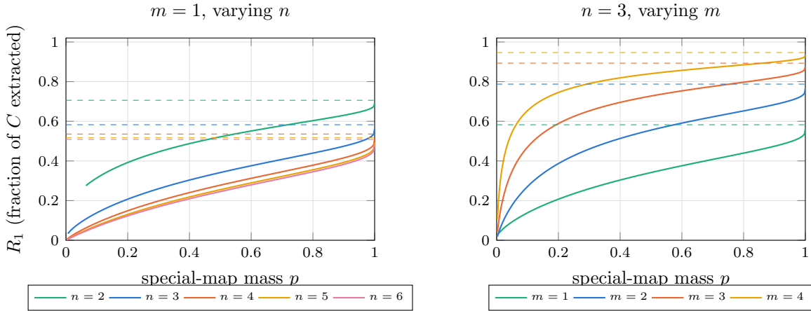
Figure 19: The exact one-question extraction ratio (127) of the spike prior, plotted only where it is defined ( 1/N < p < 1 ). Dashed lines are the exact finite- N limits (129) as p \rightarrow 1^- . Growing n drives them down to 1 - u = 1/2 ; growing m lifts them toward one.
