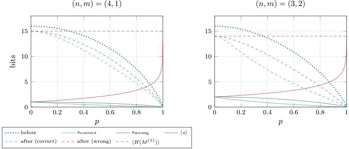
Figure 17: One-question anatomy of the spike prior against the special map's mass p : the branch surprisals (122) (solid), the answer-matrix entropy before the question (dotted) and on each branch after it (123) (dashed). Both panels carry Qm = 16 bits of table entropy at the uniform point.
