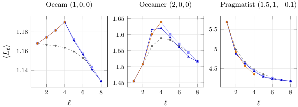
Figure 11: Expected leverage under the Gibbs priors at (3, 2), \ell^* = 4 . Greedy Werner’s fixed set is the optimal set under Occam and, up to an input negation, under Occamer. For the Pragmatist, the \ell^* – optimal has the worst leverage at the horizon, reminding that we’re optimizing for information received, while accepting that may cost even more surprisal.
