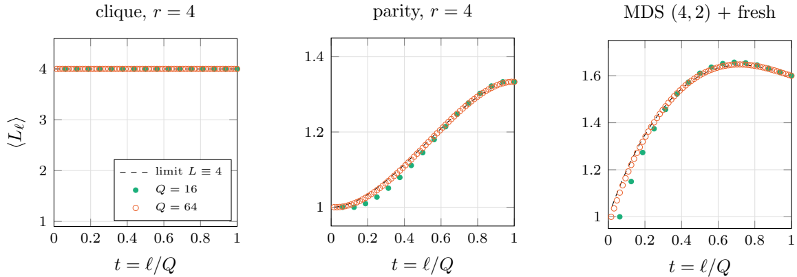
Figure 22: Exact finite- n leverage (dots, Q = 16 and 64 ) against the macroscopic limits (dashed), from (140) and (87) with no simulation. Left: cliques of four with a fair shared bit; the dots sit exactly on the constant L \equiv 4 at every finite n . Middle: parity blocks of four; deductions concentrate late and the finite curves approach the rise to r/(r-1) = \frac{4}{3} from below. Right: a 3:1 mixture of [4, 2] MDS code blocks ( m = 2 ) with fresh questions; the code releases its deductions around the threshold and the fresh sites keep receiving afterwards, an interior maximum of 1.645 at t \simeq 0.72 against the completion value 1.6.
