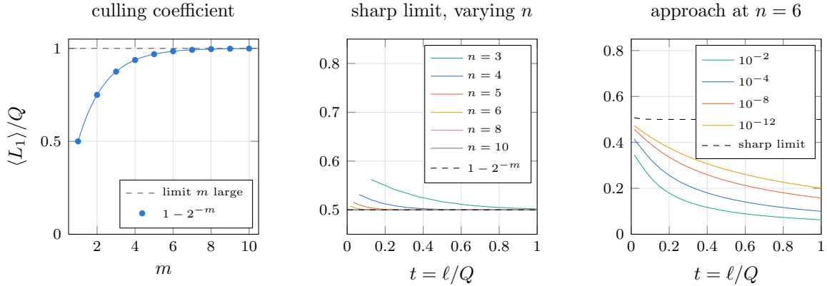
Figure 20: Left: the culling coefficient (133) against the answer width. Middle: the sharp-prior curve (132) normalized by Q , whose O(1) boundary layer is squeezed into the origin as n grows, leaving the plateau at 1 - u . Right: the approach at fixed n = 6 , m = 1 , labelled by 1 - p . Tightening the prior lifts the curve only logarithmically, so the plateau is approached pointwise in t but never uniformly.
