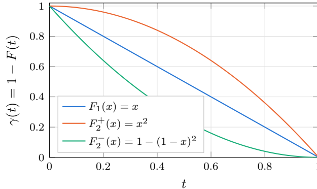
Figure 16: The profiles behind Figure 15: the survival function \gamma(t) = 1 - F(t) of each statistic, which by (101) is the mean entropy of a fresh answer at macroscopic time t . Convex, straight and concave F give concave, straight and convex profiles; the smaller of two draws spends its predictive power earliest, the larger of two hoards it.
