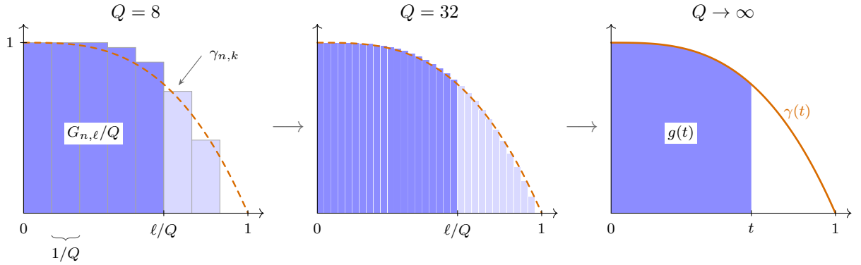
Figure 14: From the finite increments to the profile. Each bar has width 1/Q and height \gamma_{n,k} , so the shaded bars sum, the telescoping identity (97), to exactly G_{n,\ell}/Q , here at t = \ell/Q = 5/8 . Refining Q shrinks the bars onto the staircase’s limit, and dominated convergence turns the shaded sum into the area g(t) = \int_0^t \gamma : received information per question becomes the dark area under the profile.
