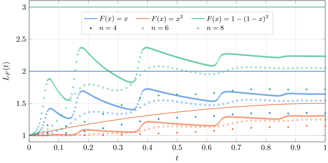
Figure 15: The three worked statistics in (94), their profiles in Figure 16. A uniform draw ( F(x) = x , blue) gives constant leverage L \equiv 2 ; the larger of two uniform draws ( F(x) = x^2 , orange) delays the deductions and the curve rises from the baseline to L(1) = \frac{3}{2} ; the smaller of two draws ( F(x) = 1 - (1 - x)^2 , green) is the r = 2 member of (96) and holds the higher constant L \equiv 3 . Dots are finite- n leverage: filled n = 4 (all 2^{16} question sets enumerated, exact), circles n = 6 and triangles n = 8 (Monte Carlo over question orders, subset entropies exact via the nested rank profile, latent-label information included). Convergence is slow from below: the label costs O(\log n) of the Q available bits, and the mean rate approaches its limit only as 1/\sqrt{n} . The left edge is a boundary layer: L_F(0^+) = 1 + f(0^+) presumes 1 \ll \ell \ll Q , while at \ell = 1 the only exhaustible class is the constants and \langle L_1 \rangle = 1 + (Q - 1) w_0^2 / (2 \ln 2) + O(w_0^3) , the early deductions being spent on identifying the latent label. The finite curves also scallop, most visibly at n = 8 : each surge is one class being learned out near its rate K_d/Q , a discreteness the limit smooths away as the rate grid refines.
