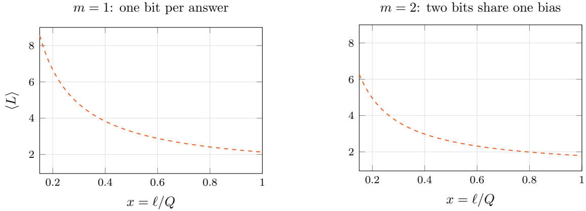
Figure 19: The same shared-scalar latent at two answer widths. Exact blocks use G_\ell = F_{m\ell} and the dashes use (??) . The curves approach their hyperbolas at every fixed x > 0 ; no uniform convergence at the singular origin is claimed.
