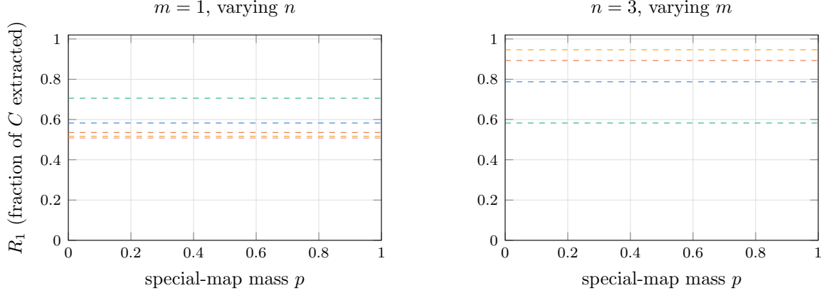
Figure 15: The exact one-question extraction ratio (??) of the spike prior, plotted only where it is defined ( 1/N < p < 1 ). Dashed lines are the exact finite- N limits (??) as p \rightarrow 1^- . Growing n drives them down to 1 - u = 1/2 ; growing m lifts them toward one.
