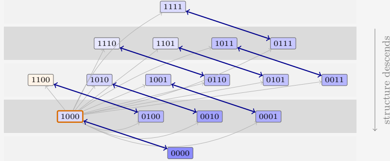
Figure 5: The update rule in the ledger, drawn for the guiding example’s first question ( q = 11 ). Every set is paired with the partner whose membership of 11 is toggled (arrows); each pair is averaged with the answer’s sign and renormalized, per equation (40). The pair \emptyset \leftrightarrow \{11\} at the orange-bordered asked set fixes the normalization and saturates the asked bias; each blue double arrow averages a pair into both of its members, and the net flow of structure is one shell down, toward M . The thin gray arrows from the asked q to every other pill remind that this sets the renormalization. The fill encodes each prior value to scale: darker is larger, orange is negative.
