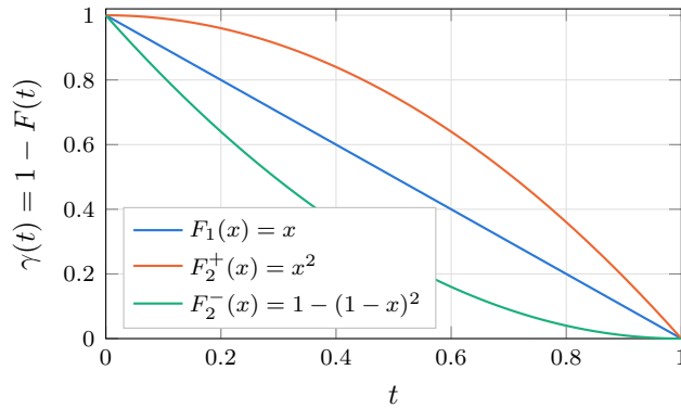
Figure 16: The increment profiles behind Figure 15: the survival function \gamma(t) = 1 - F(t) of each statistic. By (106) it is the mean entropy (expected surprisal) of one fresh answer at macroscopic time t . Convex, straight and concave F give concave, straight and convex profiles respectively; the smaller of two draws spends its predictive power earliest, the larger of two hoards it.
