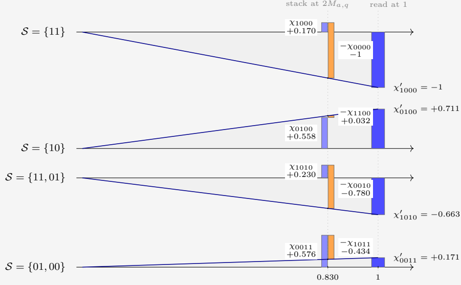
Figure 6: The update rule of equation (46), drawn for the guiding example's first update ( q = 11 , a = 1 , so (-1)^a = -1 and toggled bit 1000). One row per set \mathcal{S} . At x = 2M_{a,q} = 1 + (-1)^a \chi_{1000} = 0.830 stands the numerator as a waterfall: the bar of \chi_{\mathcal{S}} (blue), and beside it the partner's signed contribution (-1)^a \chi_{\mathcal{S} \Delta \{q\}} (orange), hanging from the level where the first bar ends. The two subscripts differ by the flipped bit. The ray from the origin through the waterfall's endpoint rescales it, by similar triangles, to x = 1 , where its height is the updated correlator \chi'_{\mathcal{S}} .
