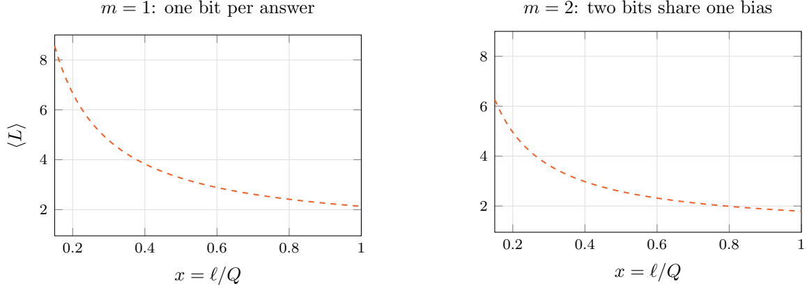
Figure 19: The same shared-scalar latent at two answer widths. Exact blocks use G_\ell = F_{m\ell} and the dashes use (105). The curves approach their hyperbolas at every fixed x > 0 ; no uniform convergence at the singular origin is claimed.
