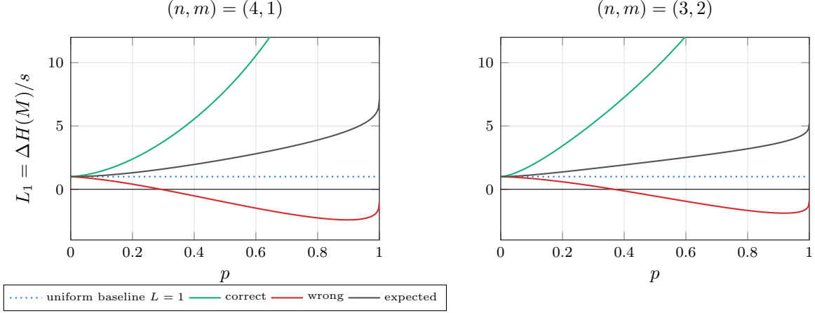
Figure 18: Branchwise (105) and expected (106) leverage of the first question. A refuting answer carries so much surprisal that its own ratio falls below the uniform baseline and eventually below zero, yet the expectation stays well above 1 because the confirming branch is both likely and cheap.
