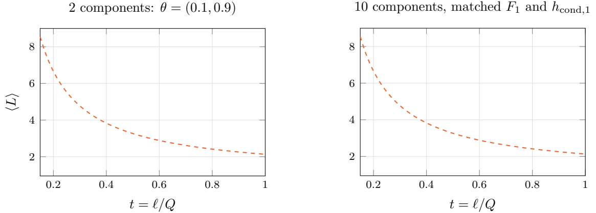
Figure 15: Two binary mixtures with the same thermodynamic curve and visibly different finite-size corrections. The right panel uses ten equally weighted biases 0.005, 0.04, 0.1, 0.2, 0.288171 and their complements, the fifth fitted so that \sum h_2 \simeq 5h_2(0.1) ; complement symmetry fixes the mean bias at \frac{1}{2} . Both therefore share h_0 = 1 and h_{\text{cond}} = h_2(0.1) , hence the same dashed hyperbola, while their finite curves differ because I_k in (81) depends on the whole collection of weights and separations. Panels begin at t = 0.15 so the common 1/t singularity does not dominate the scale.
