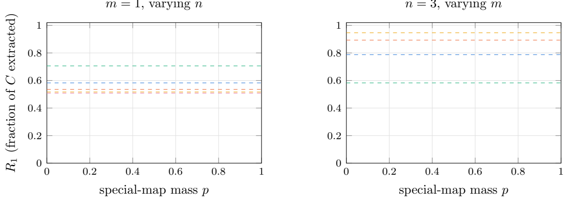
Figure 21: The exact one-question extraction ratio (125) of the spike prior, plotted only where it is defined ( 1/N < p < 1 ). Dashed lines are the exact finite- N limits (127) as p \rightarrow 1^- . Growing n drives them down to 1 - u = 1/2 ; growing m lifts them toward one.
