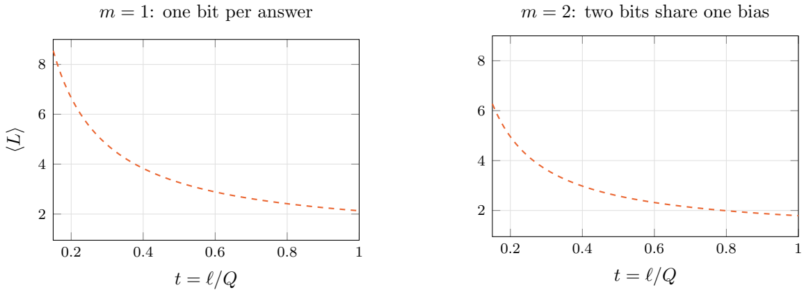
Figure 16: The same shared-scalar latent at two answer widths. Exact blocks use G_\ell = F_{m\ell} and the dashes use (92). The curves approach their hyperbolas at every fixed t > 0 ; no uniform convergence at the singular origin is claimed.
