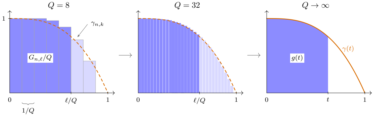
Figure 14: From the finite increments to the profile. Each bar has width 1/Q and height \gamma_{n,k} , so the shaded bars sum, the telescoping identity (88), to exactly G_{n,\ell}/Q , here at t = \ell/Q = 5/8 . Refining Q shrinks the bars onto the staircase's limit, and dominated convergence turns the shaded sum into the area g(t) = \int_0^t \gamma : received information per question becomes the dark area under the profile.
