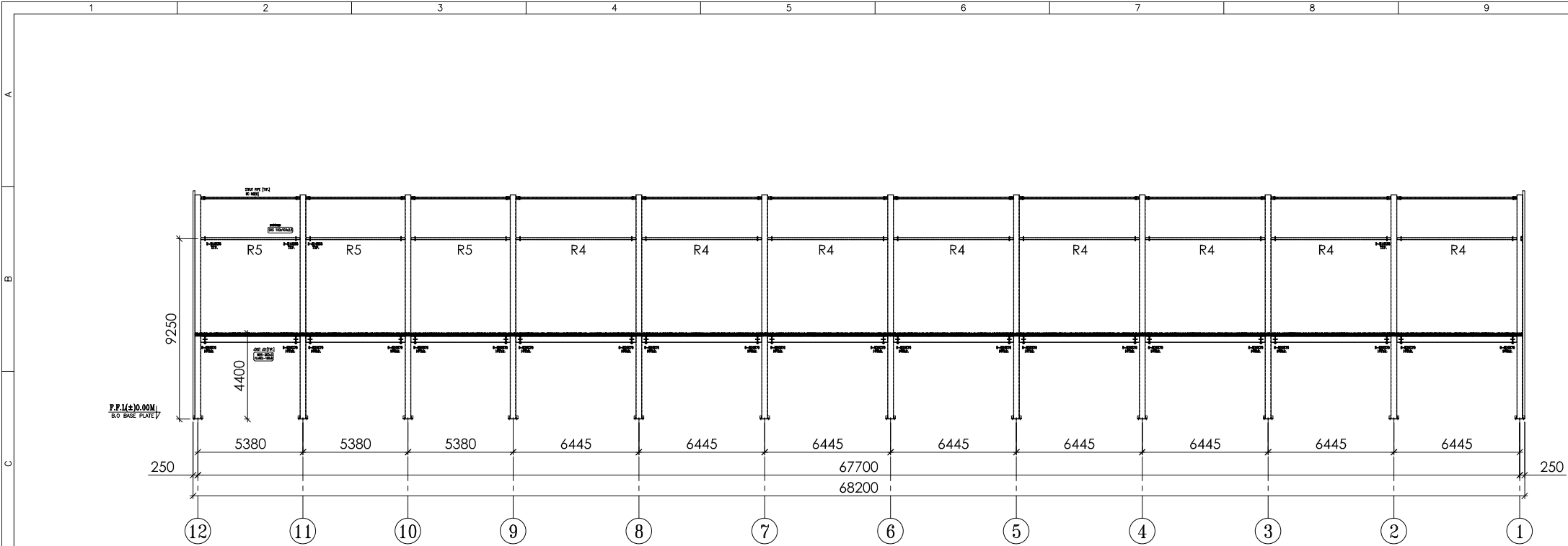
SIDE WALL FRAMING ALONG GRID - A
