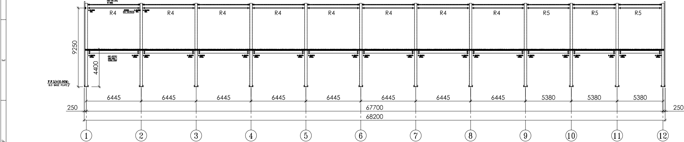
SIDE WALL FRAMING ALONG GRID - D
