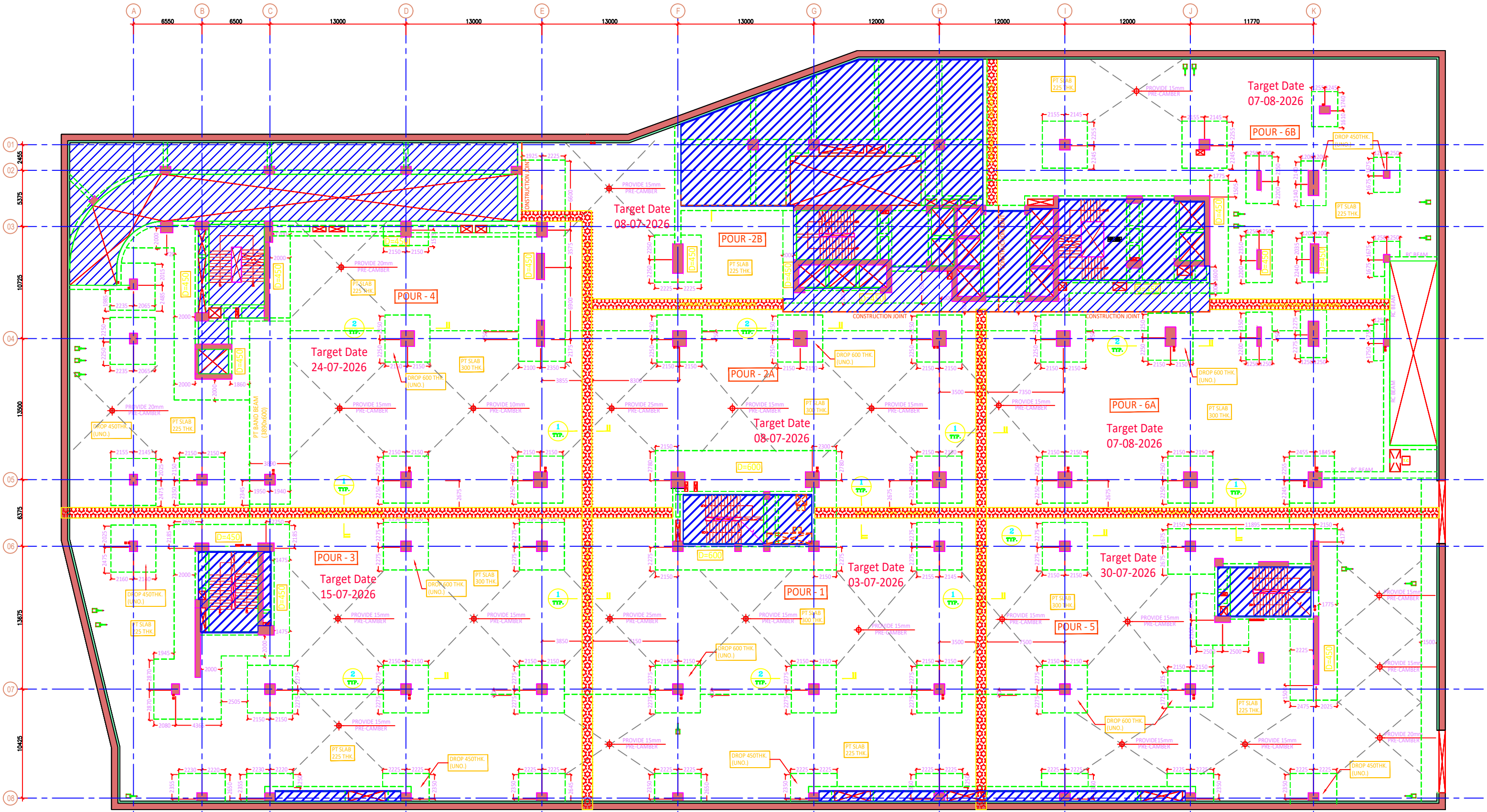
BASEMENT-2 FLOOR (TYPE 1) LEVEL PT SLAB - FORMWORK LAYOUT PLAN
