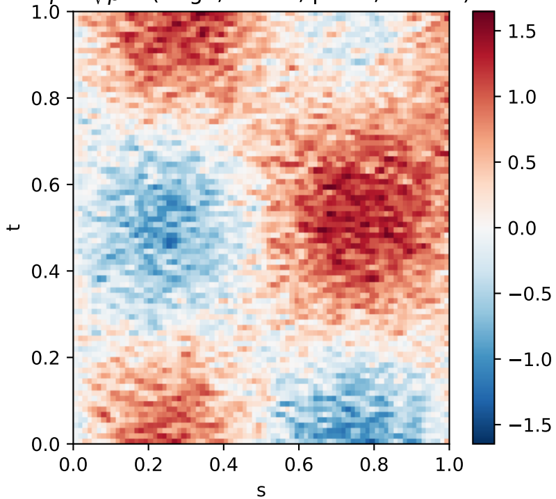
\hat{\beta} = \sqrt{p} \hat{B} (ridge, \lambda=4.6 , p=80 , n=500 )
