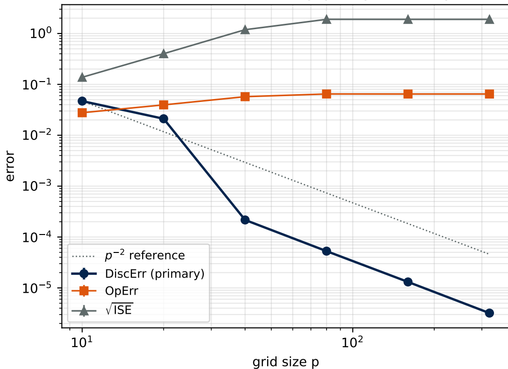
Sweep A: discretization gap vs grid density
